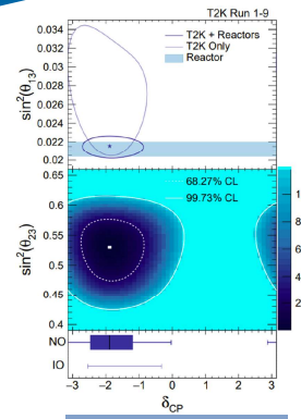
T2K CP violation
