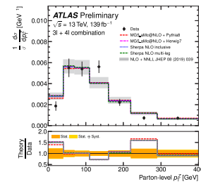
ATLAS Differential ttZ
