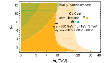
CLIC top compositeness
