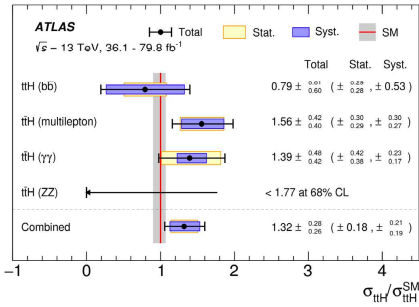
ATLAS ttH Observation
