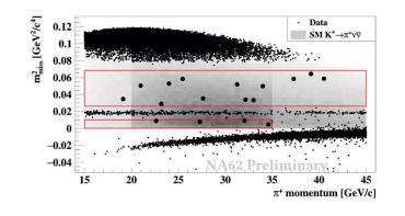
NA62 Evidence for K^+ \rightarrow \pi^+ \nu \bar{\nu}
