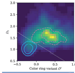
Jet colour ring VHBb
