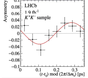
LHCb CP violation B_s^0
