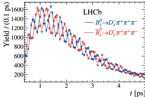
LHCb measurement \Delta m_s
