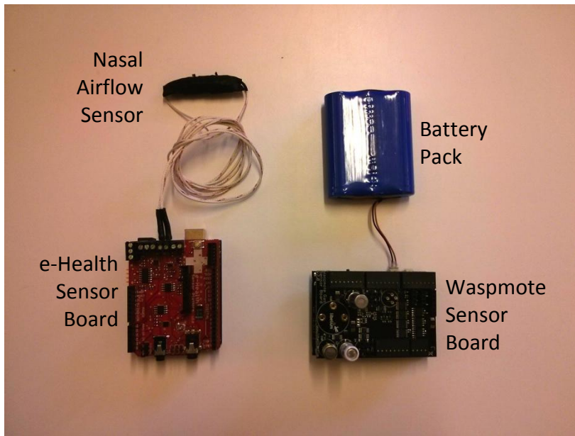
Figure 1. The Cooking Hacks e-Health sensor boards for airflow (left), and the Libelium Waspnote Gases sensor board for pollution (right).
